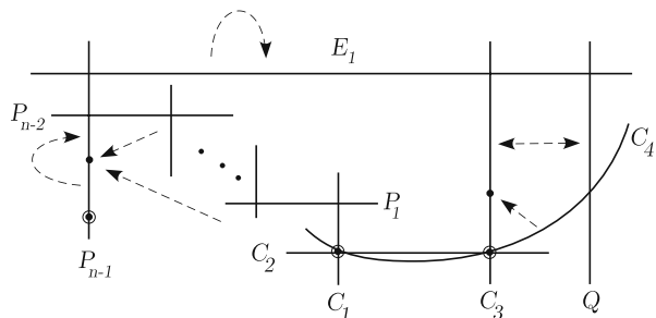
Fig. 3 The space \mathcal{X} and the action of k_{\mathcal{X}}
