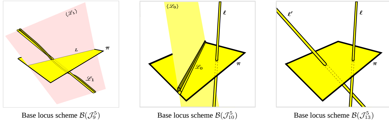
FIGURE 6. Pictorial representations (in yellow) of the base locus schemes of quadro-quadric Cremona transformations of \mathbb{P}^4 of type II.
