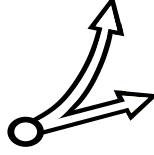
FIGURE 3. Pictorial representation of \eta
